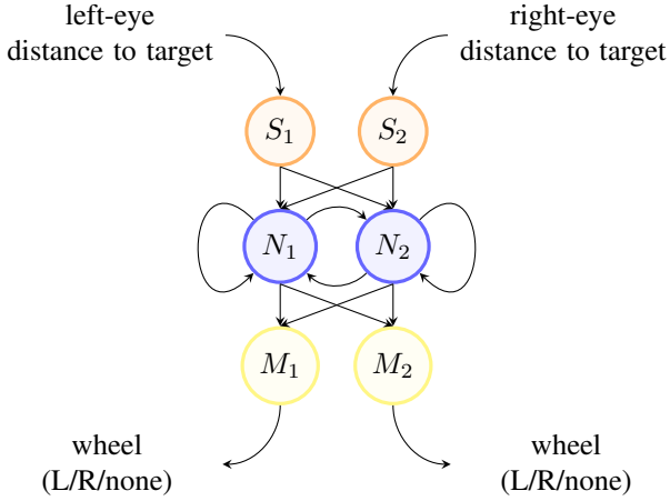
Figure 2: Network architecture: S_1, S_2 are sensory nodes, N_1, N_2 are inner nodes (brain), M_1, M_2 are motor nodes.
